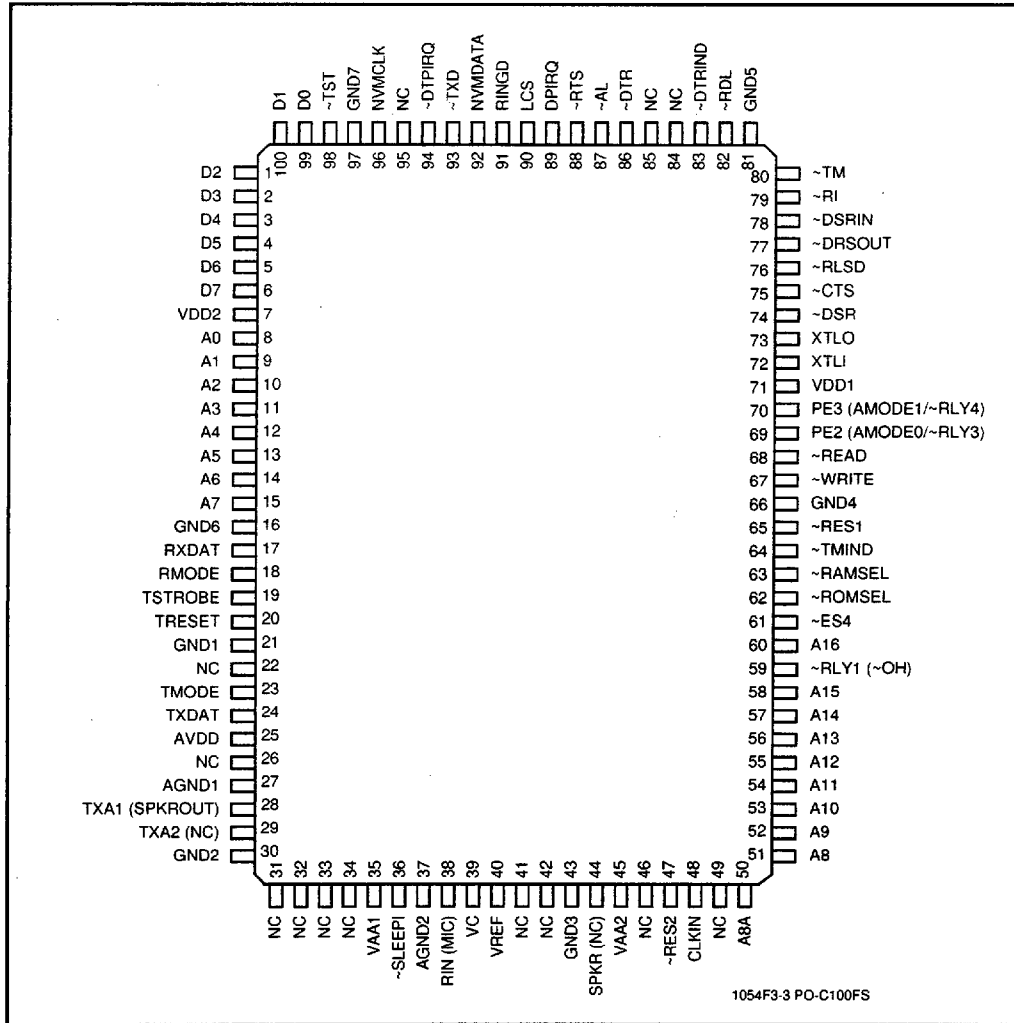
Figure 4. MCU Pin Signals - 100-Pin PQFP - Serial DTE Interface
