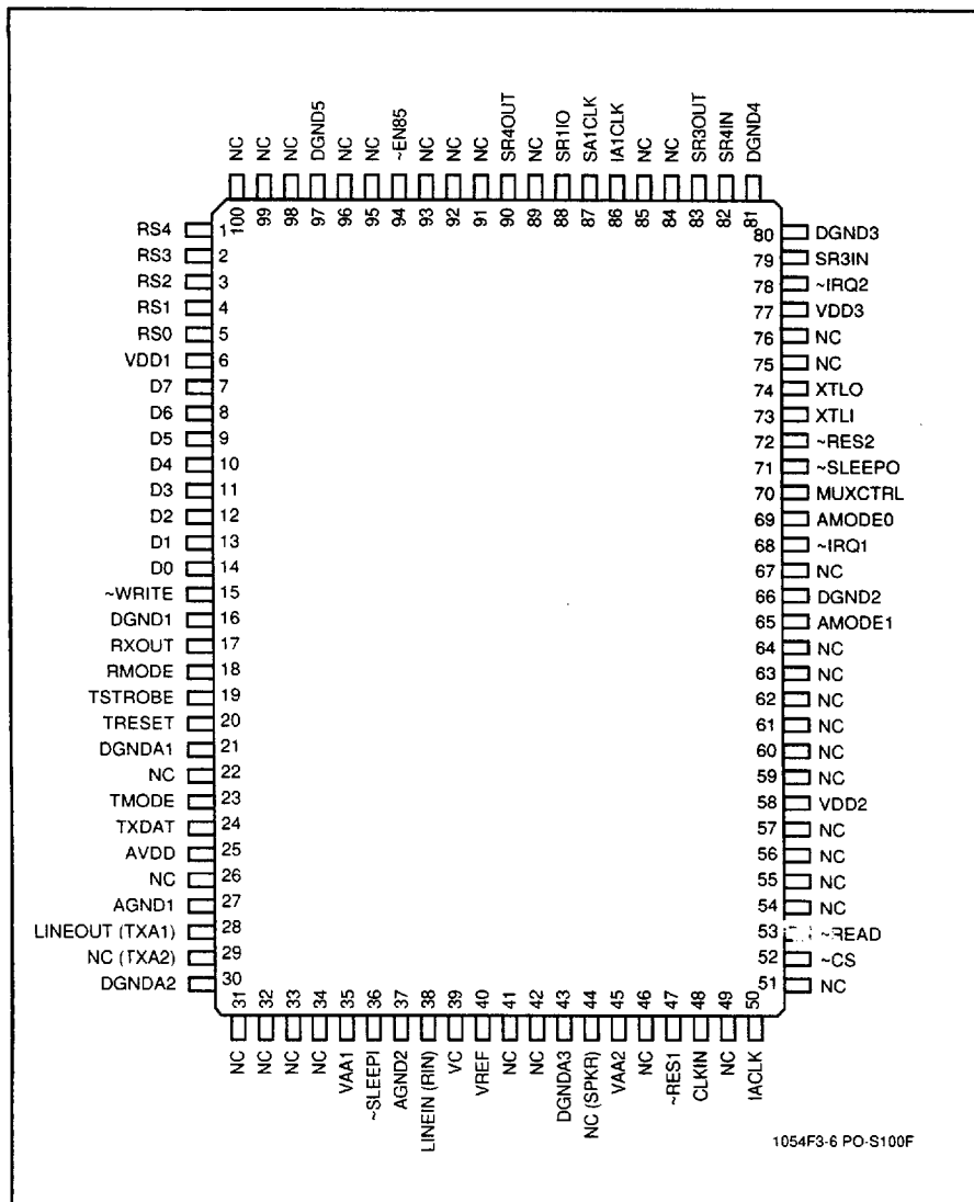
Figure 7. DTP Device Pin Signals - 100-Pin PQFP
