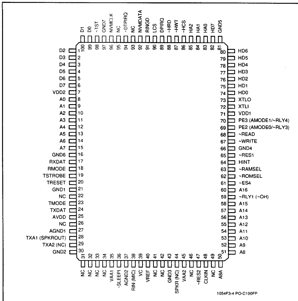
Figure 5. MCU Pin Signals - 100-Pin PQFP - Parallel Host Interface
