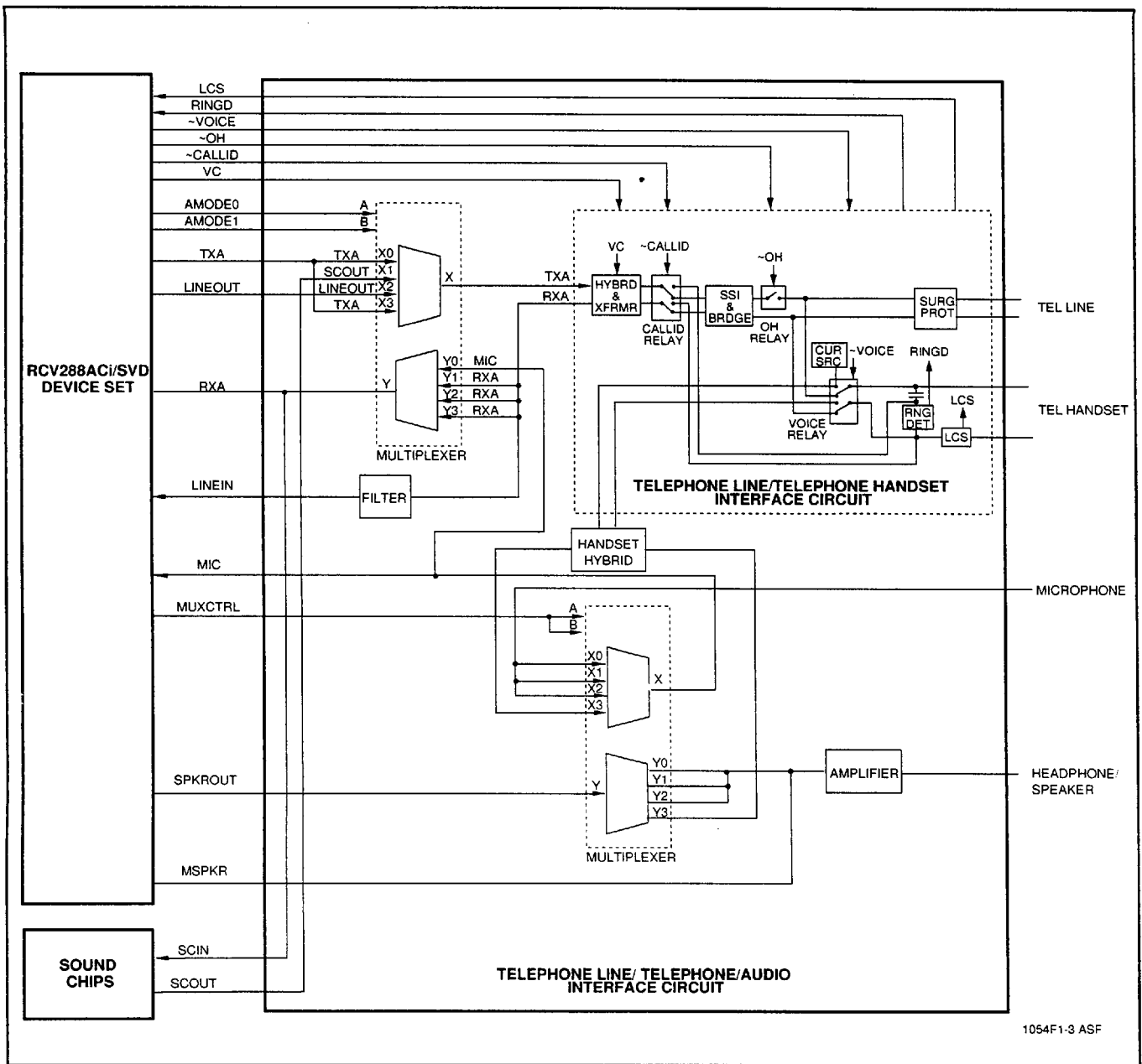
Figure 3. Audio Signal Interface
